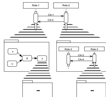
Figure 2. Interaction protocols can be specified in more detail (i.e., leveled) using a combination of diagrams.
