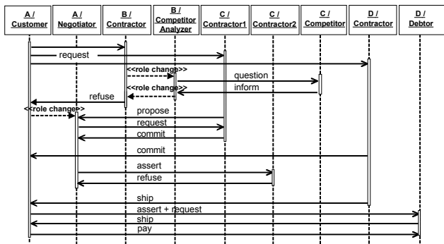
Figure 10. A sequence diagram version of Fig. 9.
