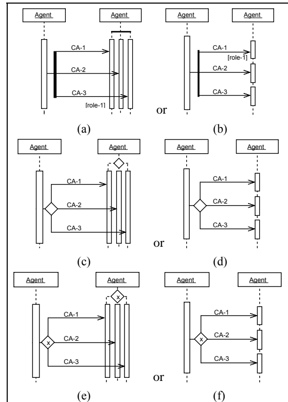
Figure 8. Multiple techniques to express concurrent communication with an agent playing multiple roles or responding to different CAs.
