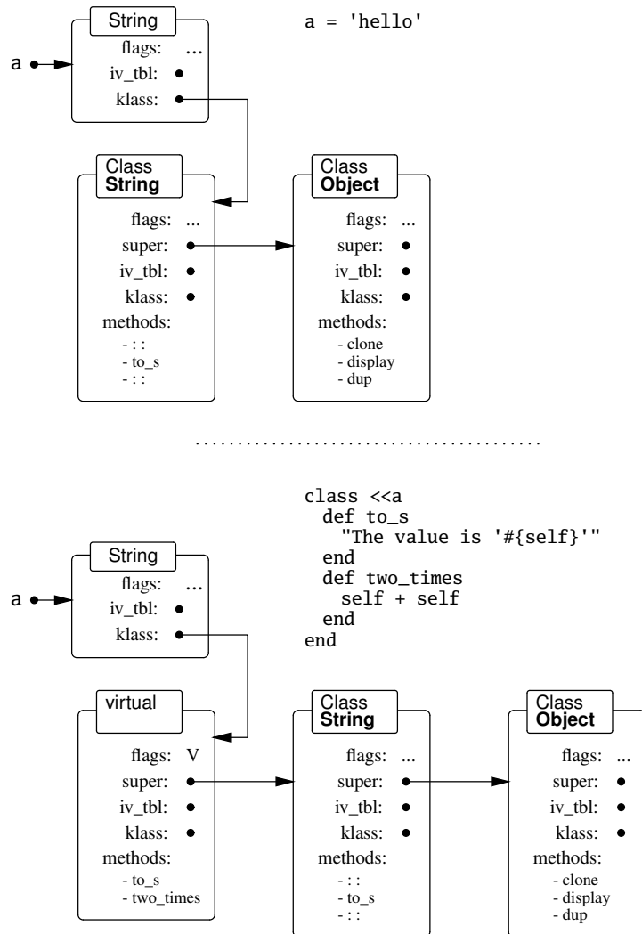
Figure 24.3. Adding a virtual class to an object
