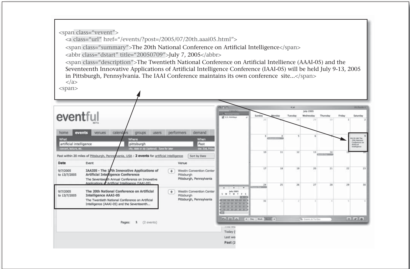
Figure 6. The hCalendar Microformat.
