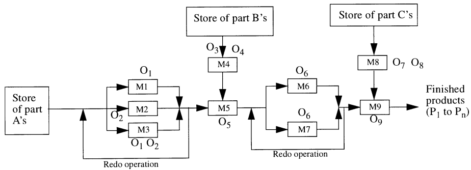
Fig. 2. Exemplar flexible manufacturing system.
